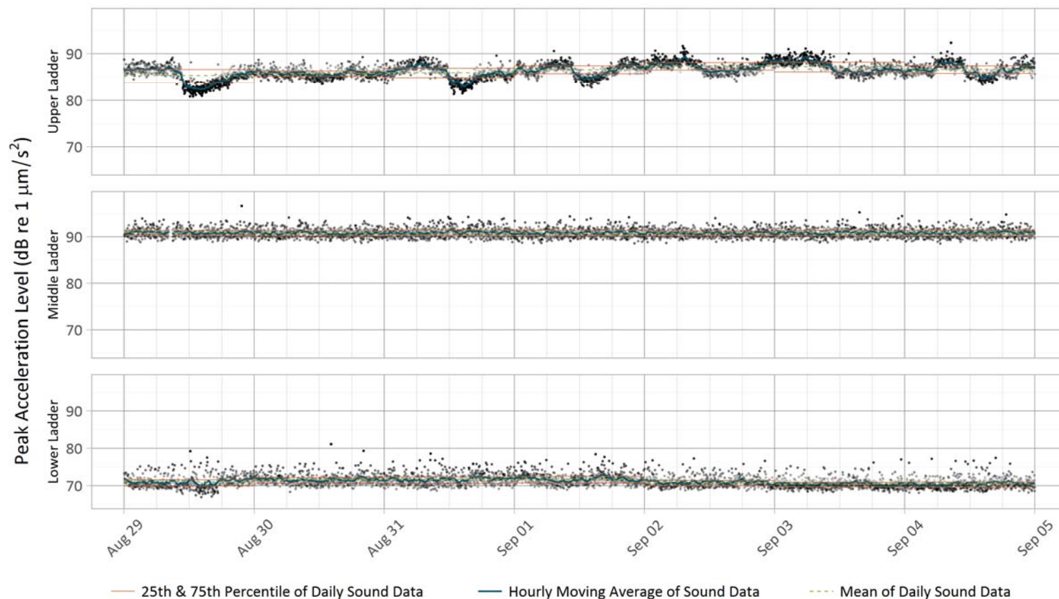
Figure 1 Peak Acceleration Levels Measured by Triaxial Accelerometers for Week 35
