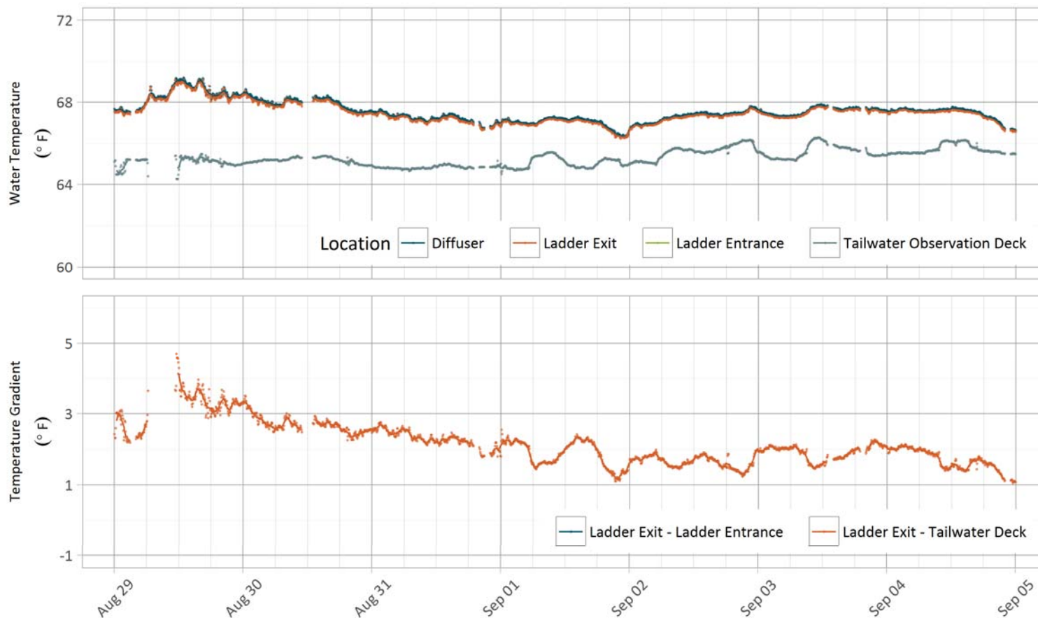
Figure 3 Water Temperatures in the Fish Ladder for Week 35
