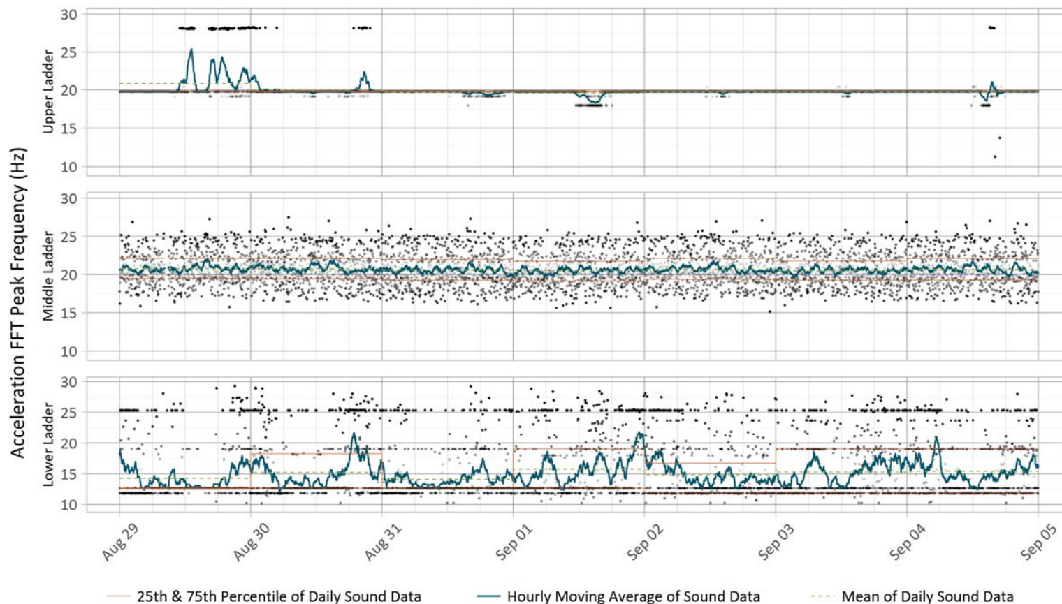
Figure 2 Acceleration Peak Frequencies Measured by Triaxial Accelerometers for Week 35
